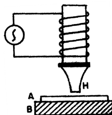
Fig. 7.7 Ultrasonic drilling
