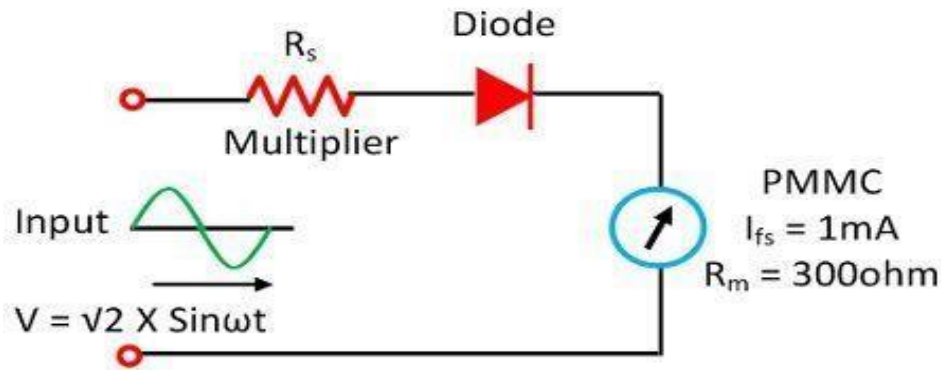
Half Wave Rectifier Circuit
