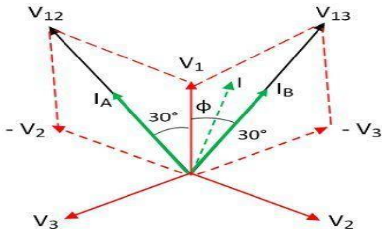
Phasor Diagram of Three Phase Electrodynamic Type Power Factor Meter
