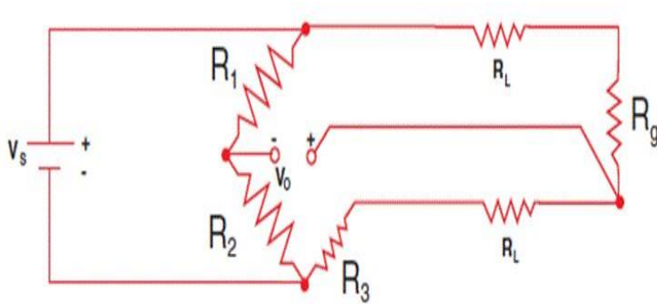
Fig.6. Circuitry view of three wires RTD Bridge
