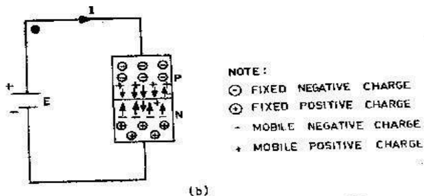
Fig. 2.6(b) The operation of PN junction under forward bias
